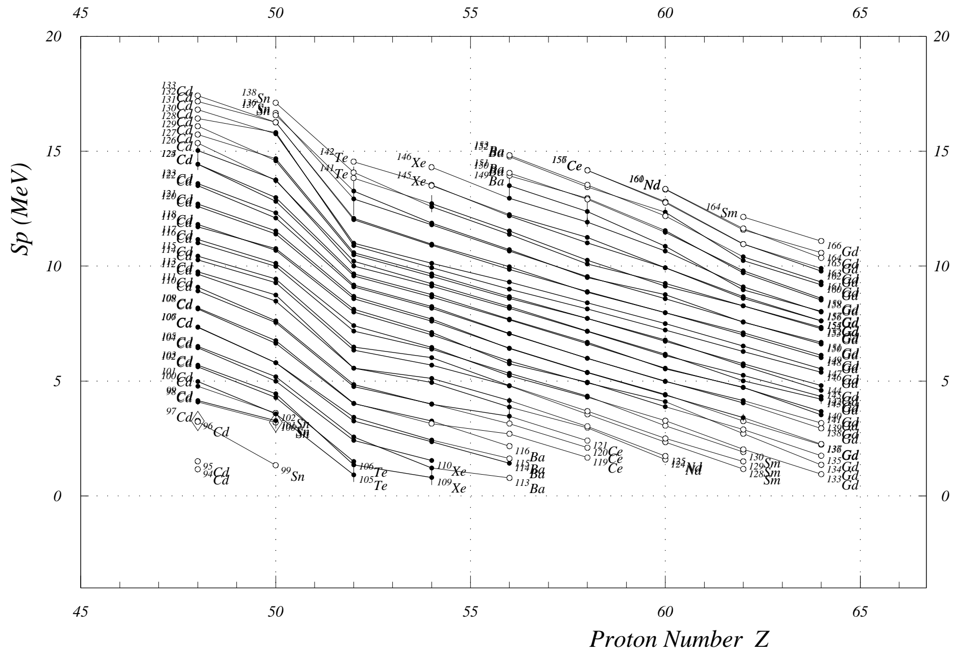
Fig. 4. One-Proton Sep. Energies (even Z) Z = 47 to 65
