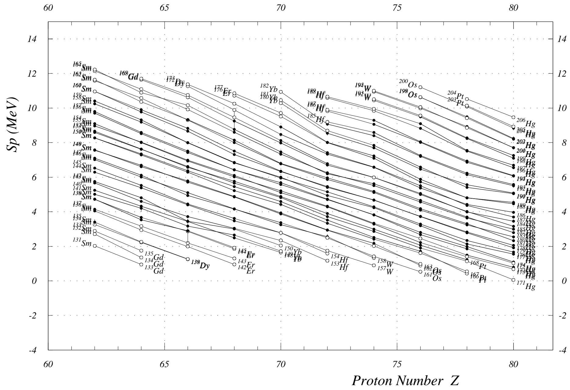
Fig. 5. One-Proton Sep. Energies (even Z) Z = 62 to 80
