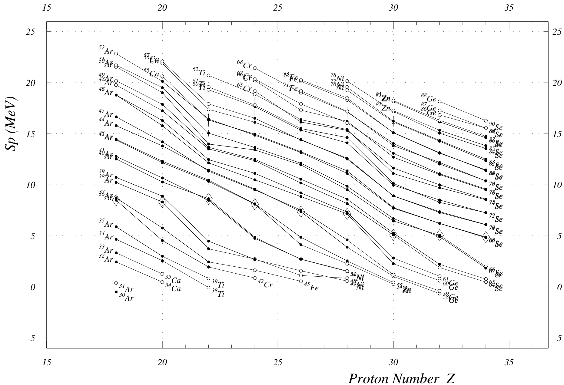
Fig. 2. One-Proton Sep. Energies (even Z ) Z = 17 to 35
