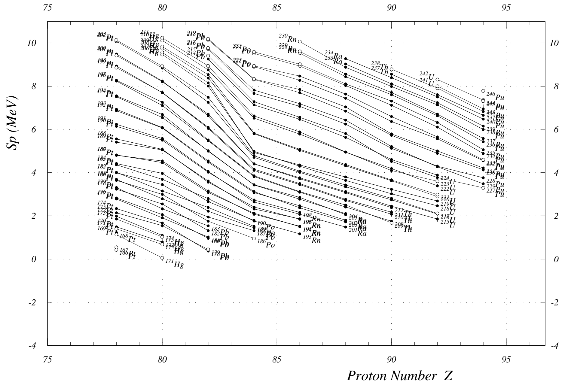
Fig. 6. One-Proton Sep. Energies (even Z) Z = 77 to 95
