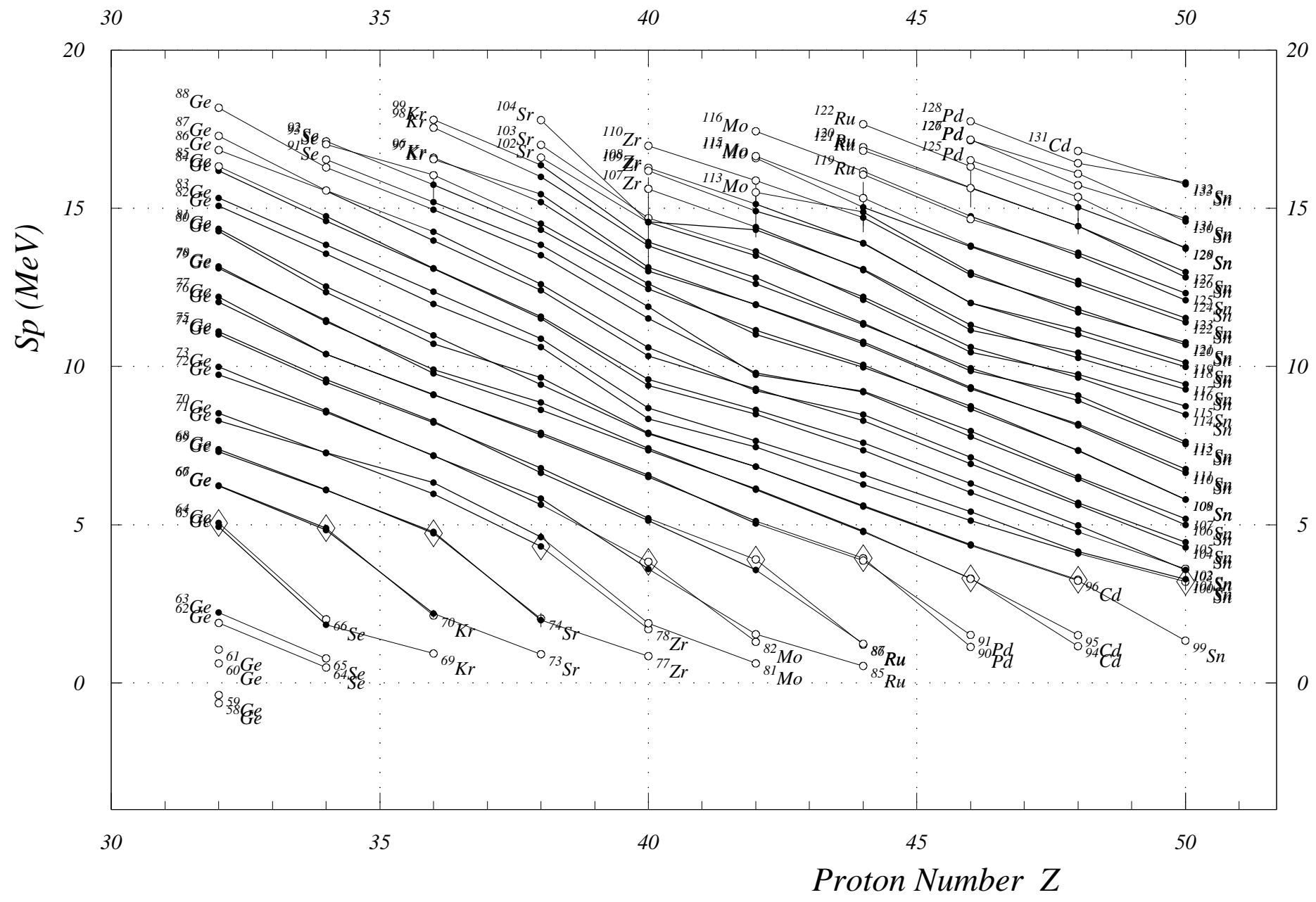
Fig. 3. One-Proton Sep. Energies (even Z) Z = 32 to 50
