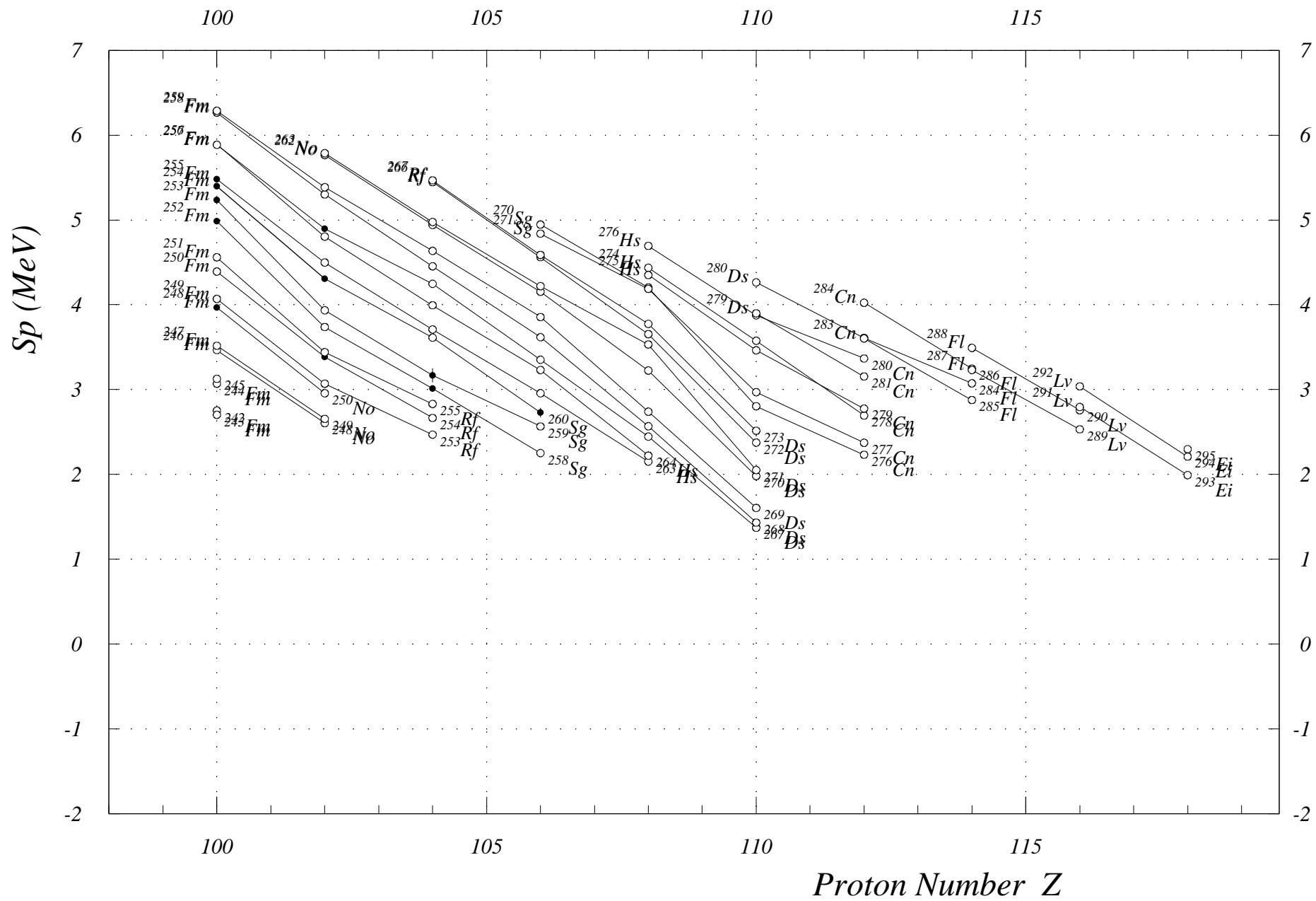
Fig. 8. One-Proton Sep. Energies (even Z) Z = 100 to 118
