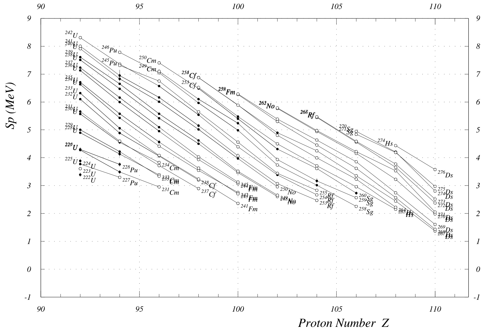
Fig. 7. One-Proton Sep. Energies (even Z) Z = 92 to 110
