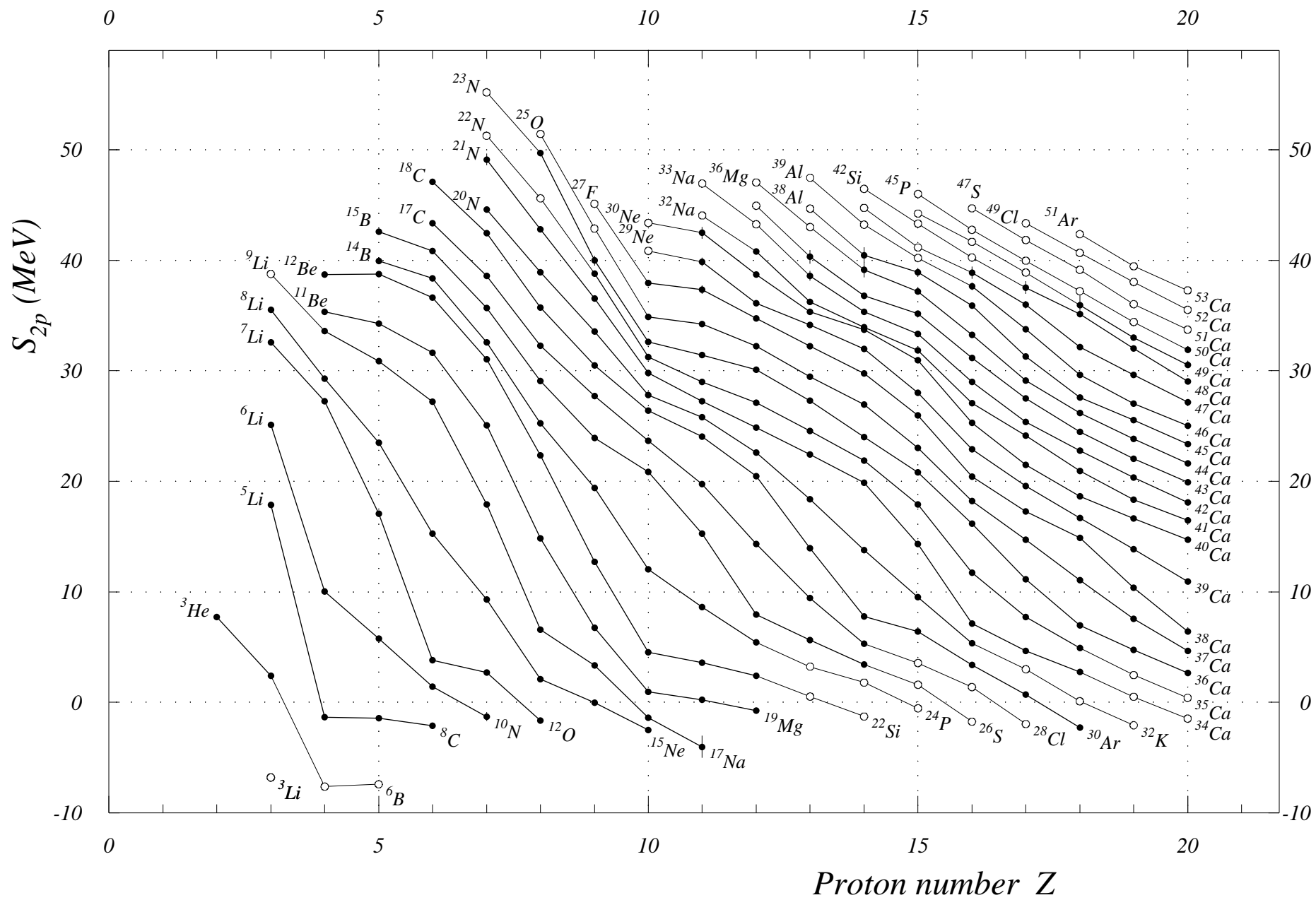
Fig. 10. Two-proton separation energies Z = 0 to 20
