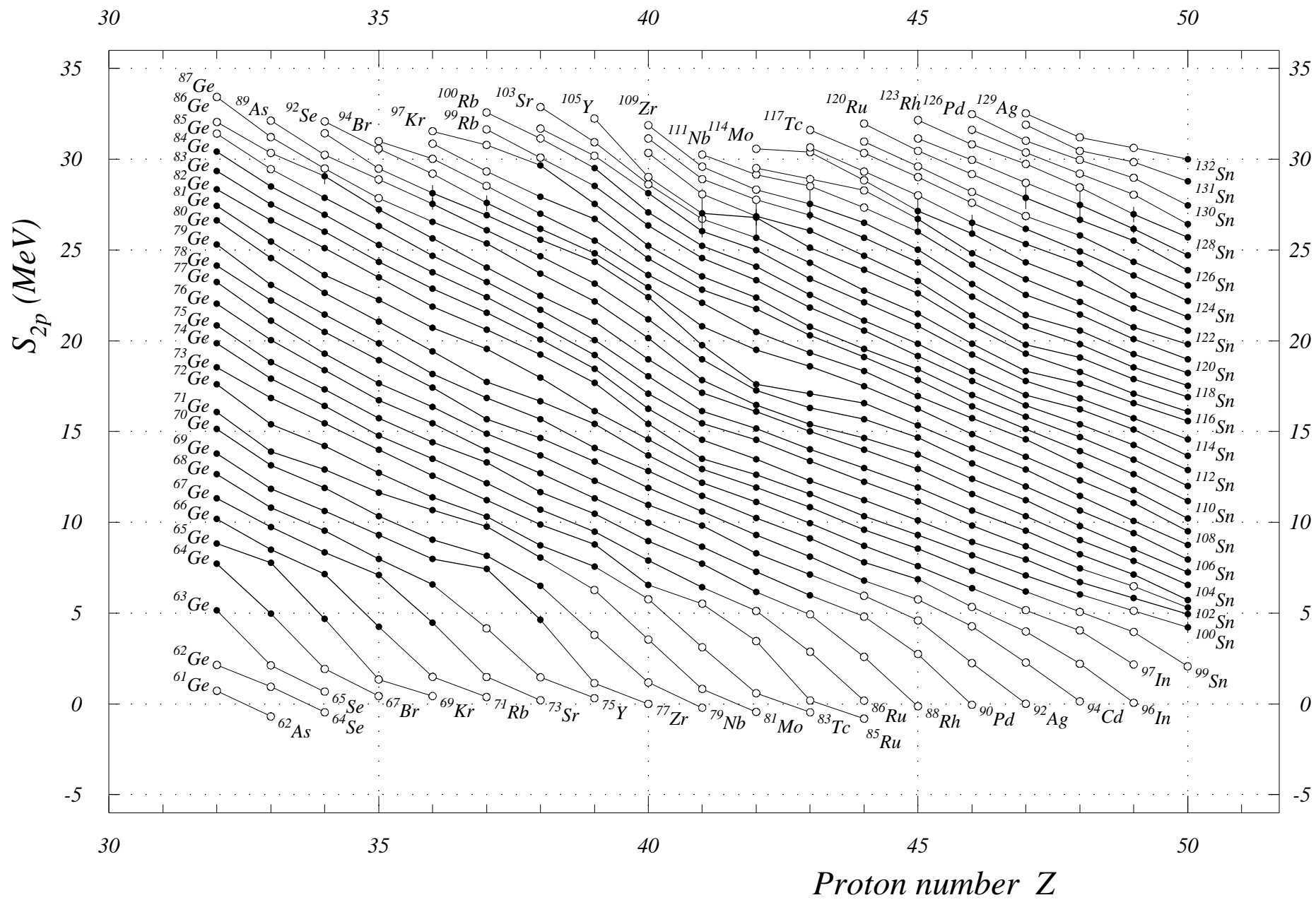
Fig. 12. Two-proton separation energies Z = 32 to 50
