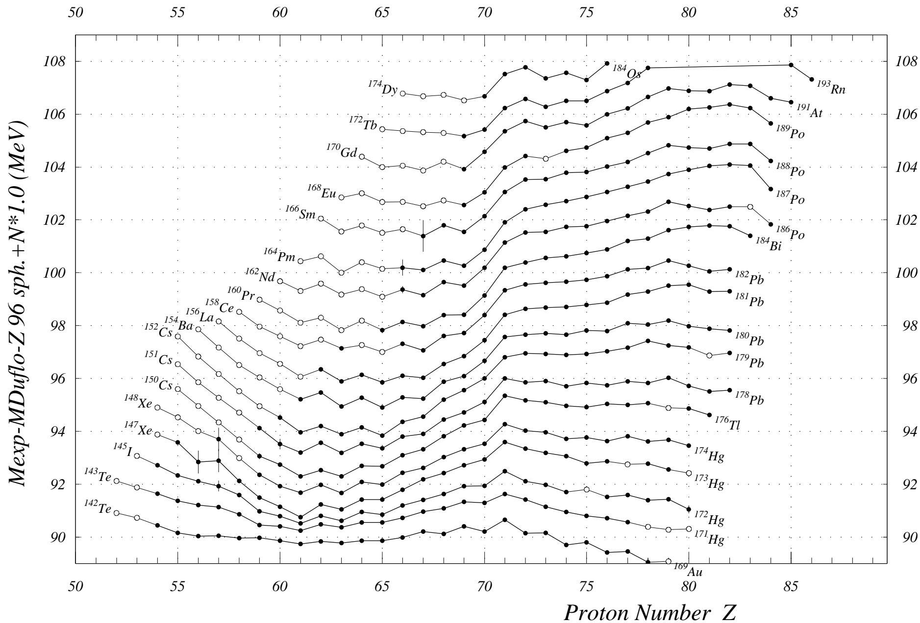
Fig. 7. Mass Exp-Mass Duflo-Z 96 sph. Z= 52 to 88
