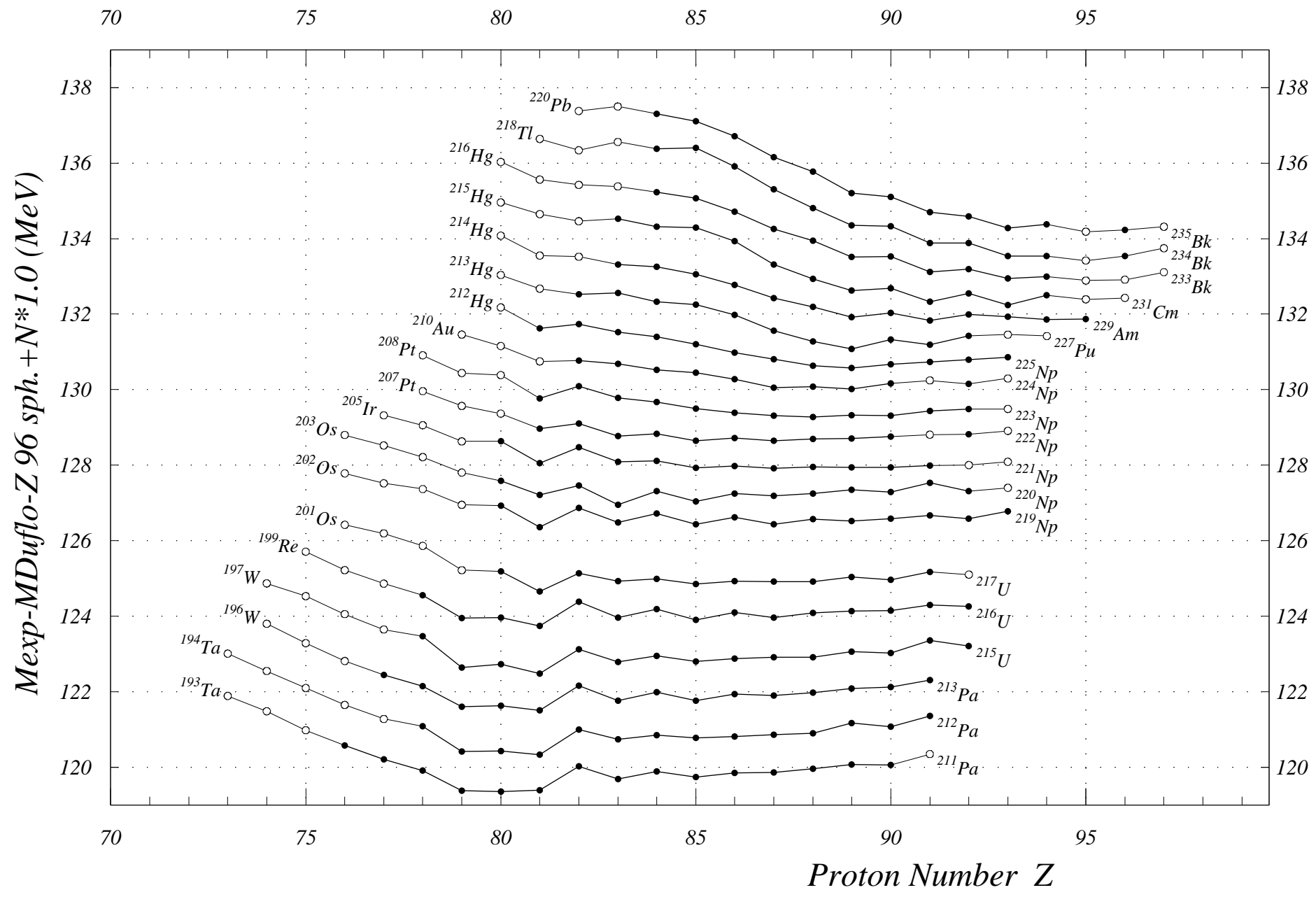
Fig. 9. Mass Exp-Mass Duflo-Z 96 sph. Z= 72 to 98
