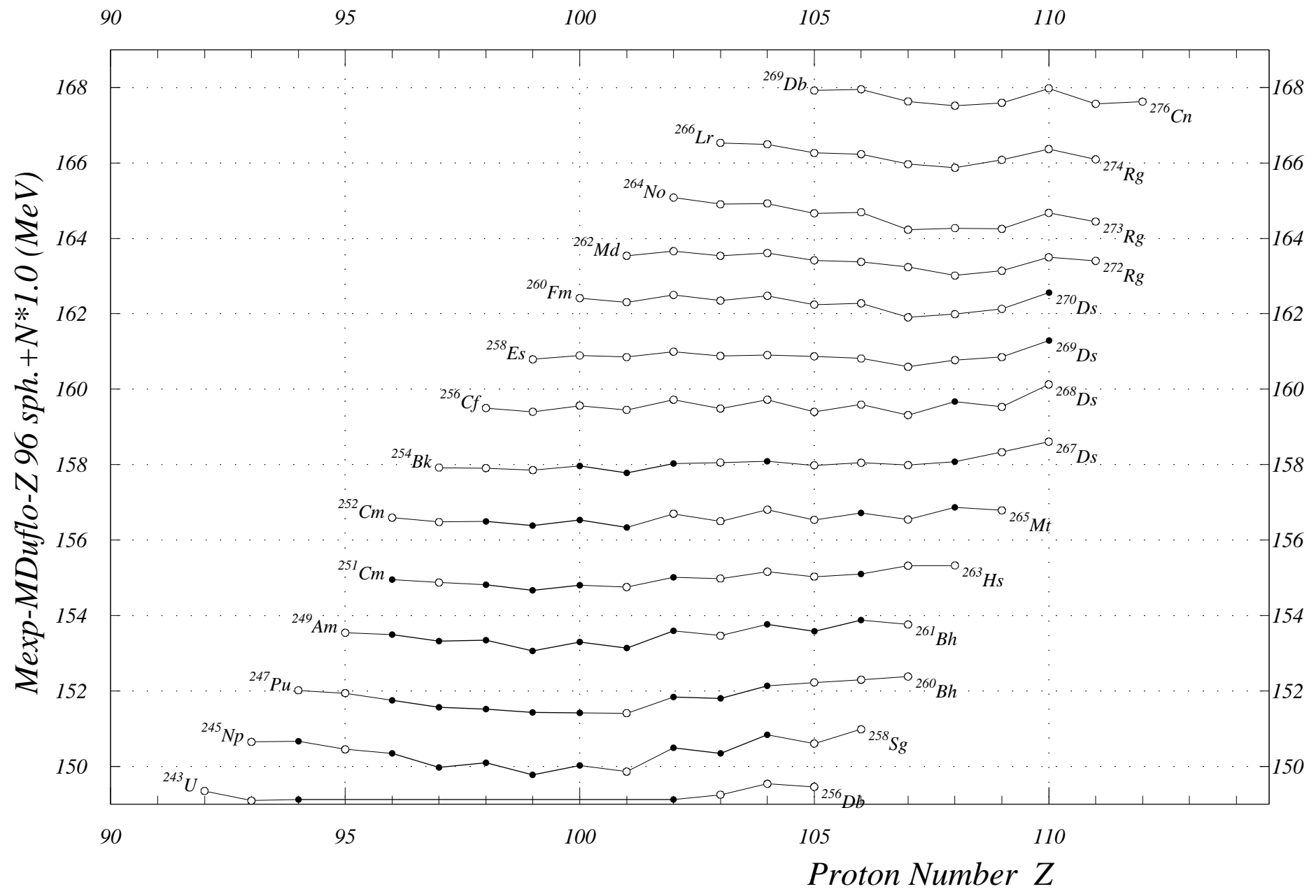
Fig. 11. Mass Exp-Mass Duflo-Z 96 sph. Z= 92 to 113
