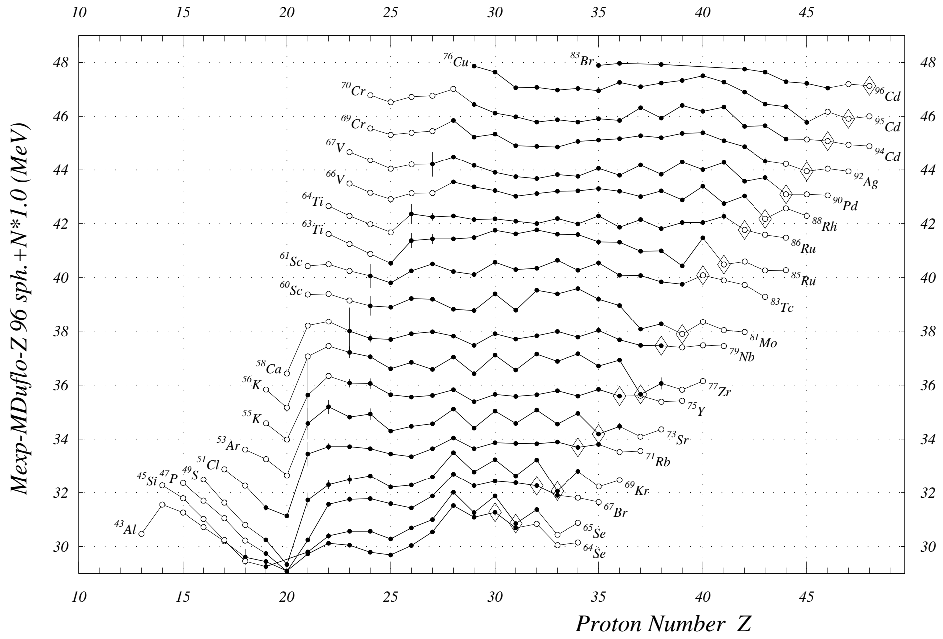
Fig. 3. Mass Exp-Mass Duflo-Z 96 sph. Z= 12 to 48
