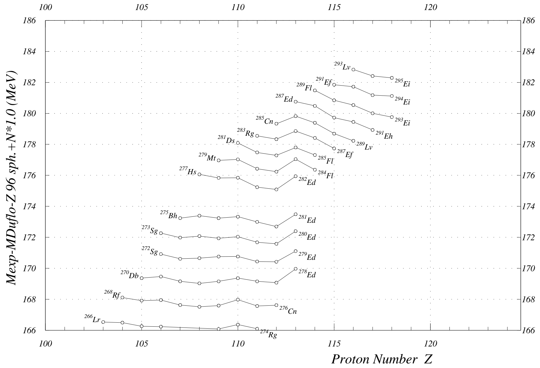
Fig. 12. Mass Exp-Mass Duflo-Z 96 sph. Z= 102 to 123
