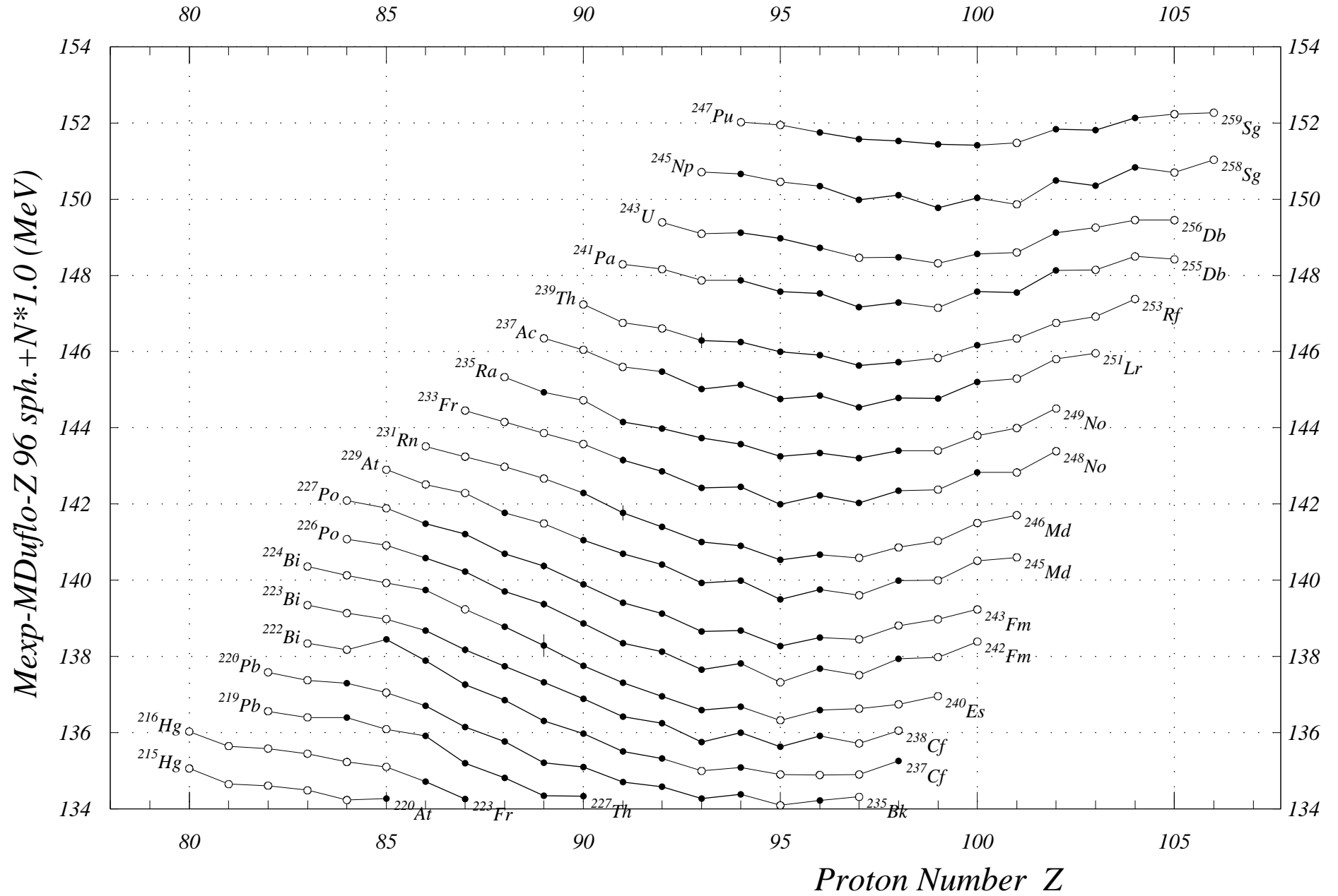
Fig. 10. Mass Exp-Mass Duflo-Z 96 sph. Z= 80 to 106
