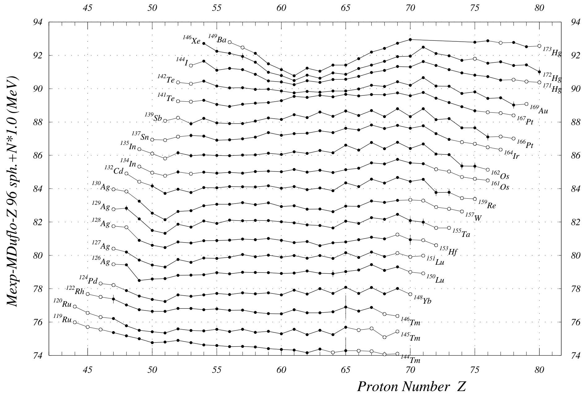
Fig. 6. Mass Exp-Mass Duflo-Z 96 sph. Z= 44 to 80
