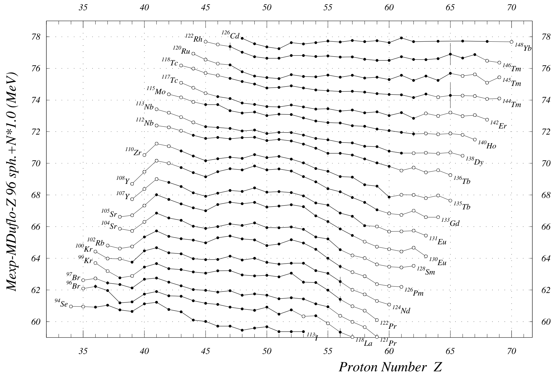
Fig. 5. Mass Exp-Mass Duflo-Z 96 sph. Z= 34 to 70
