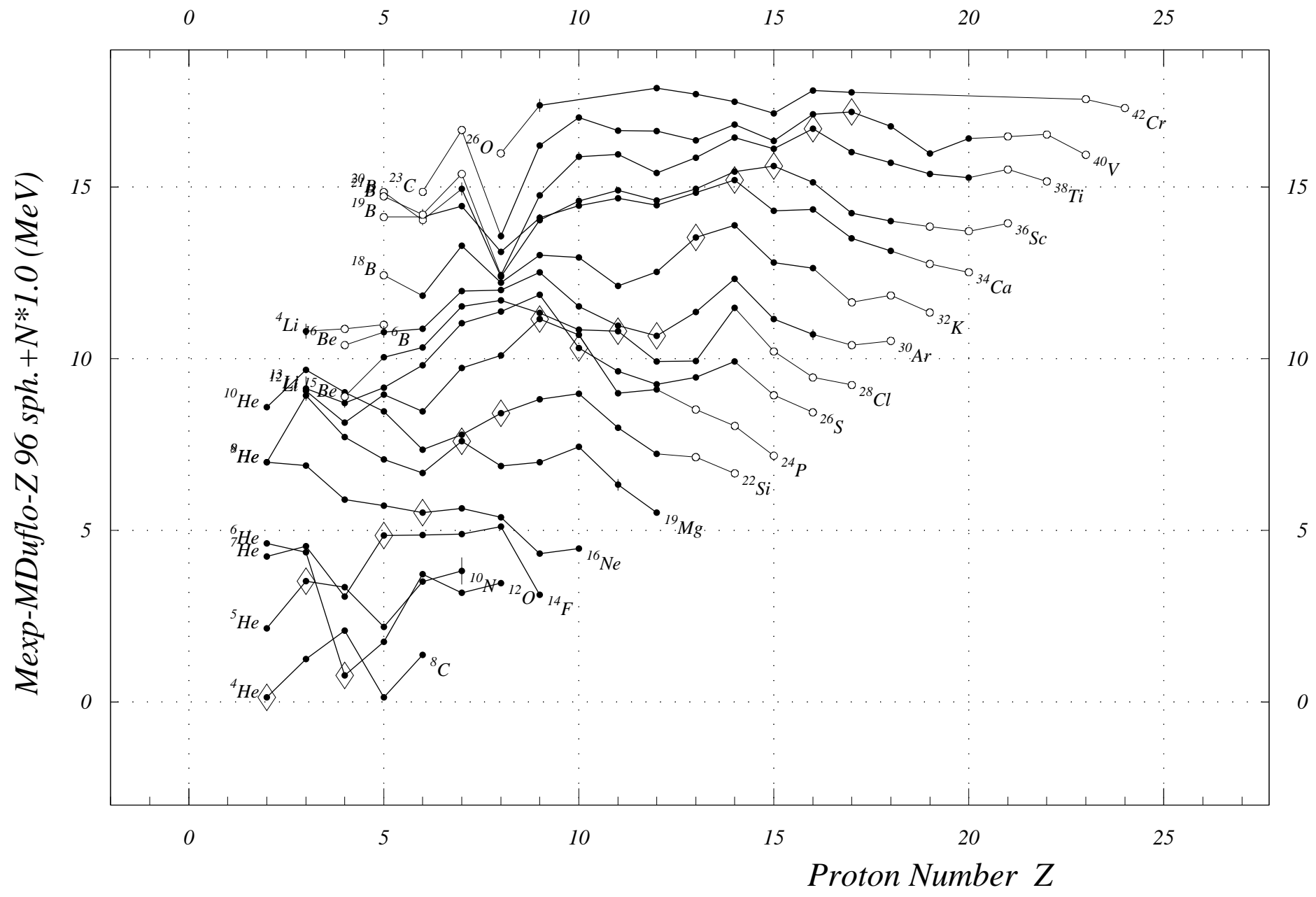
Fig. 1. Mass Exp-Mass Duflo-Z 96 sph. Z= 0 to 26
