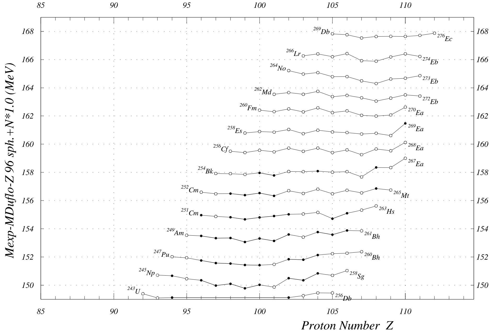
Fig. 11. Mass Exp-Mass Duflo-Z 96 sph. Z= 87 to 113
