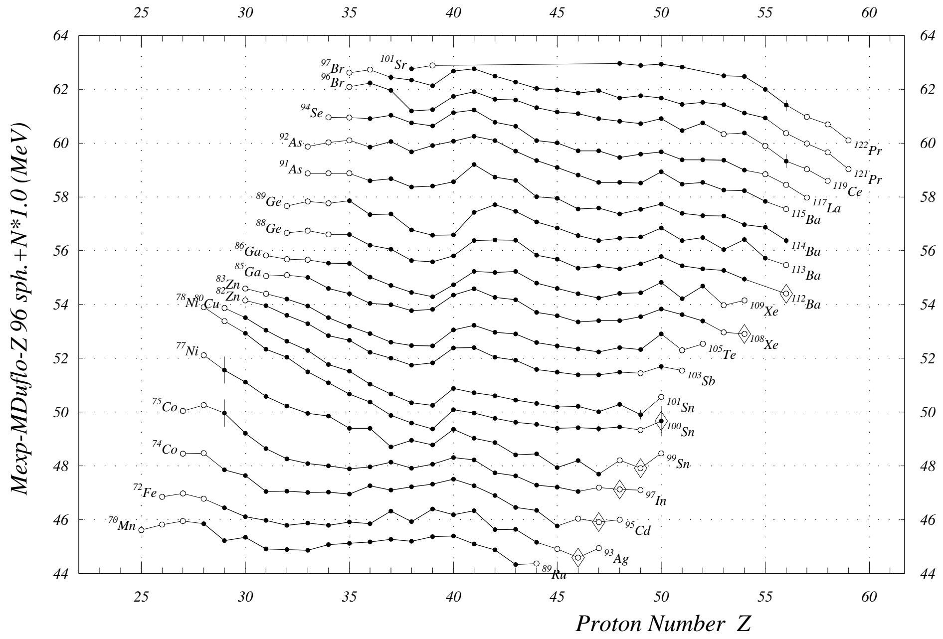
Fig. 4. Mass Exp-Mass Duflo-Z 96 sph. Z= 24 to 60
