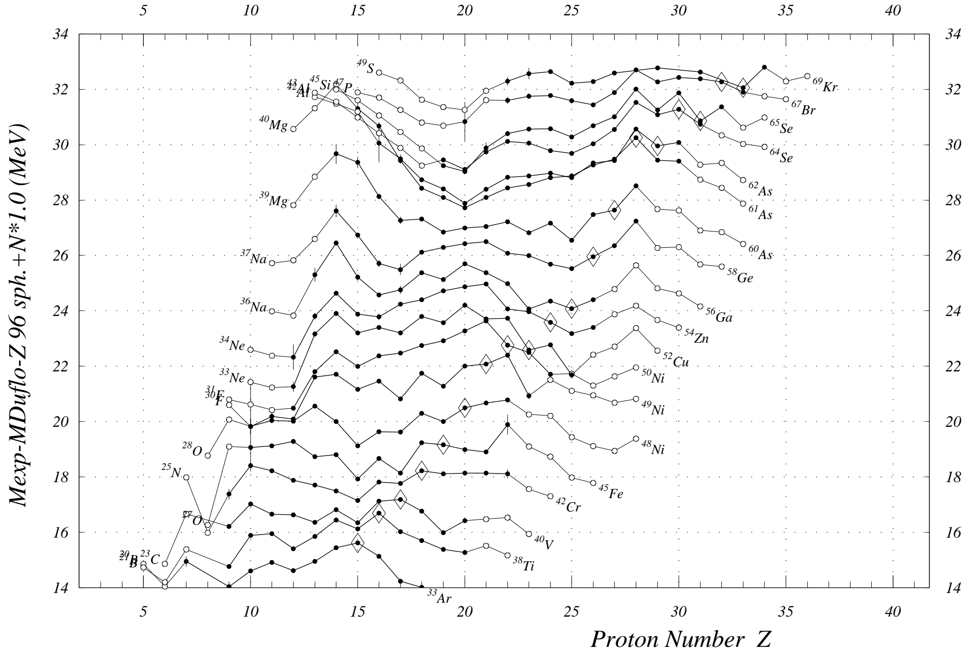
Fig. 2. Mass Exp-Mass Duflo-Z 96 sph. Z= 4 to 40
