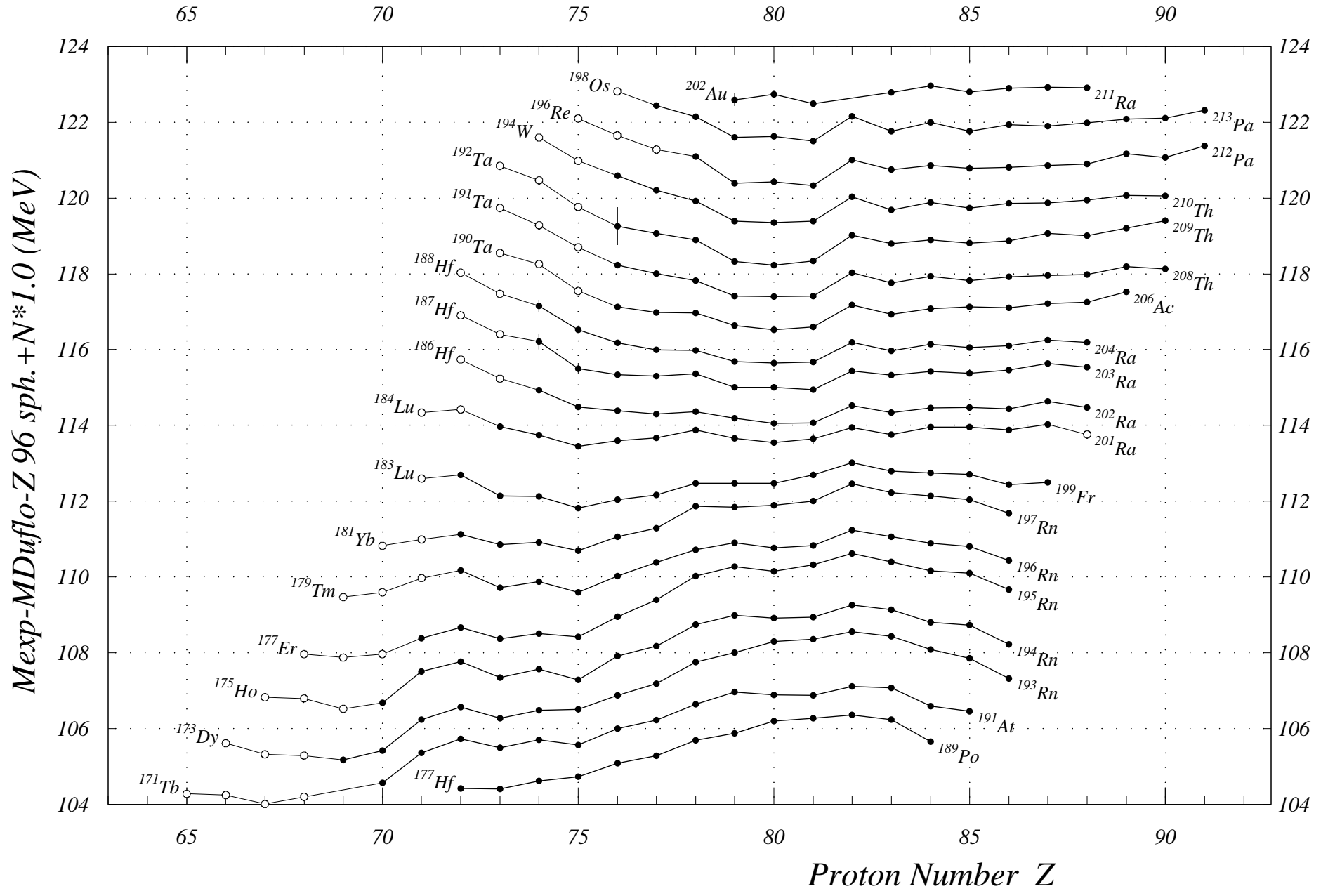
Fig. 8. Mass Exp-Mass Duflo-Z 96 sph. Z= 65 to 91
